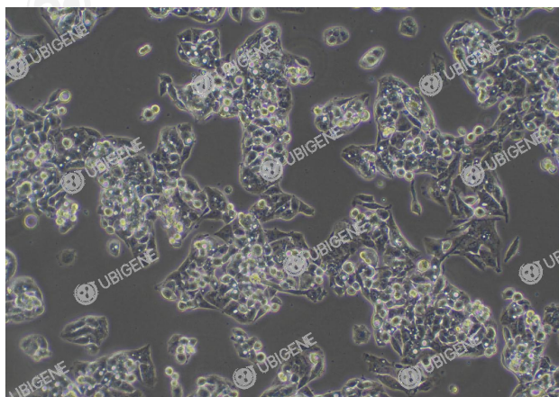
NR1H4 Stable Expression Cell Line (Hep G2)-100X
