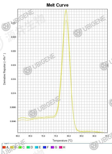
HepG2_Ctrl(Puro)+hNR1H4-1 melt curve
