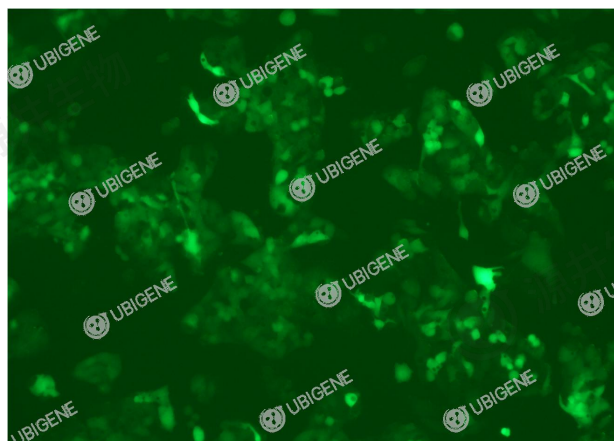
NR1H4 Stable Expression Cell Line (Hep G2)-100X-300ms
